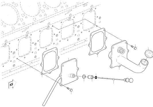
OIL FILLER NECK UPC.06G04 1455
